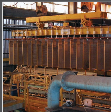
Festoon System on an Electrowinning Process Crane, Chile
