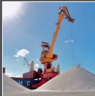
Motor Driven Cable Reel on a Ship Unloader, France
