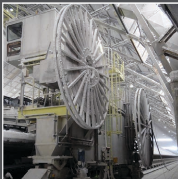
Motor Driven Cable and Hose Reels on a Tripper Conveyor, Venezuela
