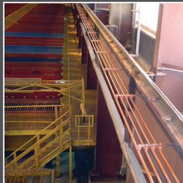
"Dura Coat" Conductor Bar System on an Electro-winning Process Crane, Chile
