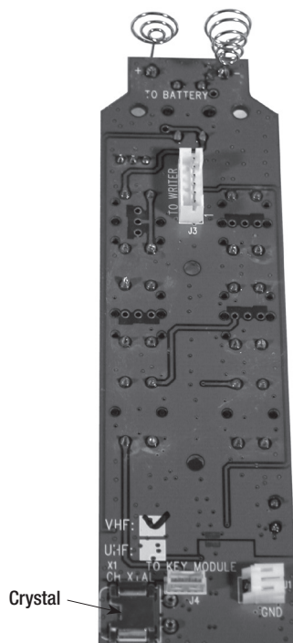
Transmitter Circuit Board (Protean HT & L8 Models)
