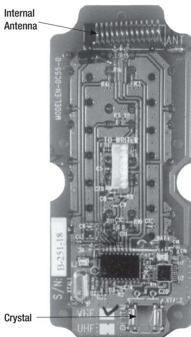
Transmitter Circuit Board (Protean 4, 6, & 8 Button)
