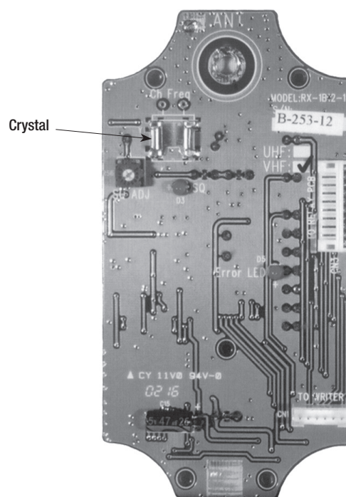
Receiver Circuit Board (All Models)
