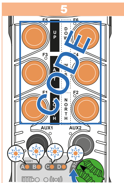
If LEDs A, B, C, and D flash at the same time, the transmitter is locked by a protection sequence. Re-enter the sequence (buttons F1-F6 ) and validate by turning the ON/OFF switch to START . If the code is correct, initialization starts (the green LED lights up for 2 sec).
